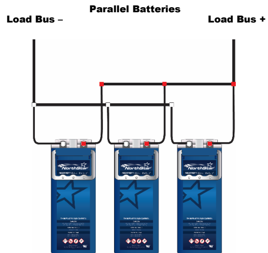
Figure 7 Parallel String Configuration
